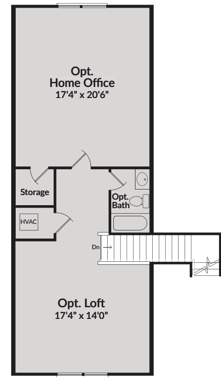
Optional Finished Loft Floorplan
