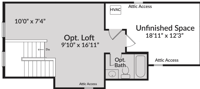
Optional Partially Finished Loft Floorplan
