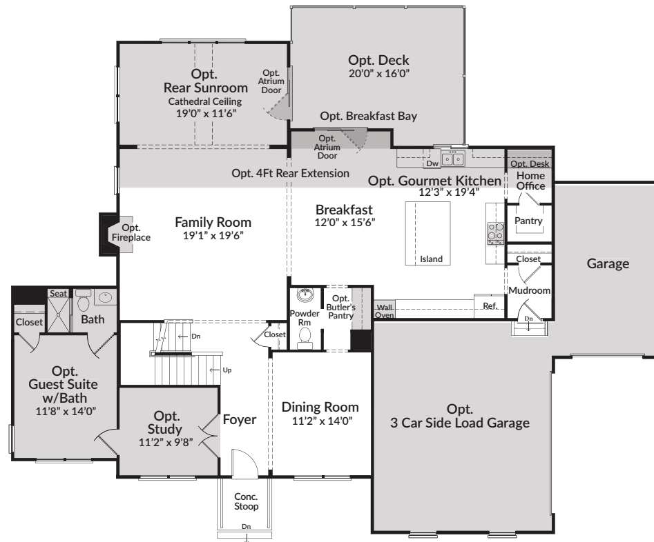
Optional Main Level Floorplan
