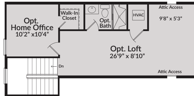
Optional Finished Loft Floorplan
