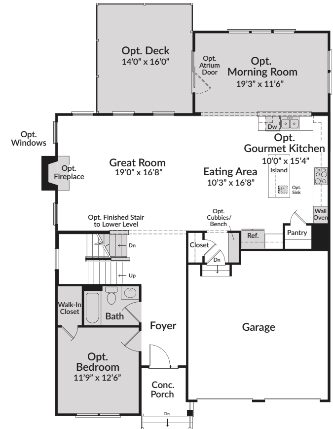
Optional Main Level Floor Plan
