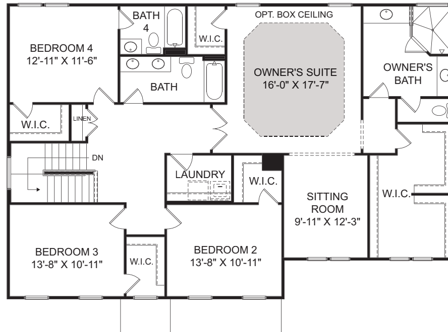
Second Level Floorplan
