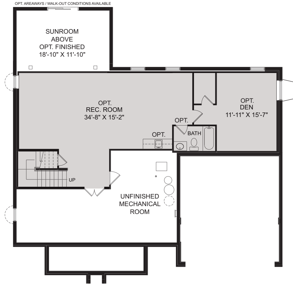
Lower Level Floorplan
