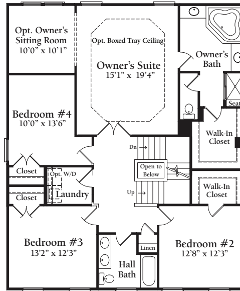
Optional Upper Level Floor Plan w/Opt. 2' Rear Extension, Opt. Boxed Tray Ceiling, Opt. Owner's Sitting Room, Stairs to Optional Loft
