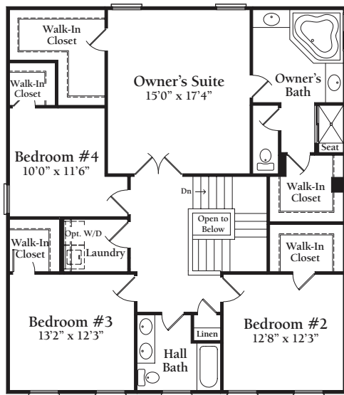
Standard Upper Level Floor Plan
