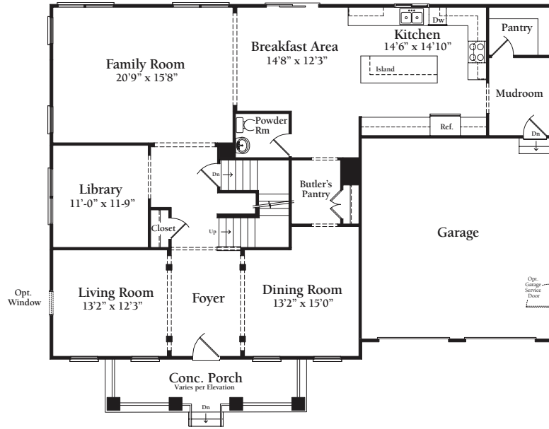
Standard Main Level Floor Plan
