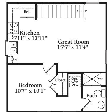
Optional Carriage House w/Opt. Finished Upper Level
