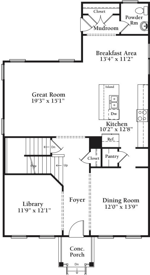
Standard Main Level Floor Plan
