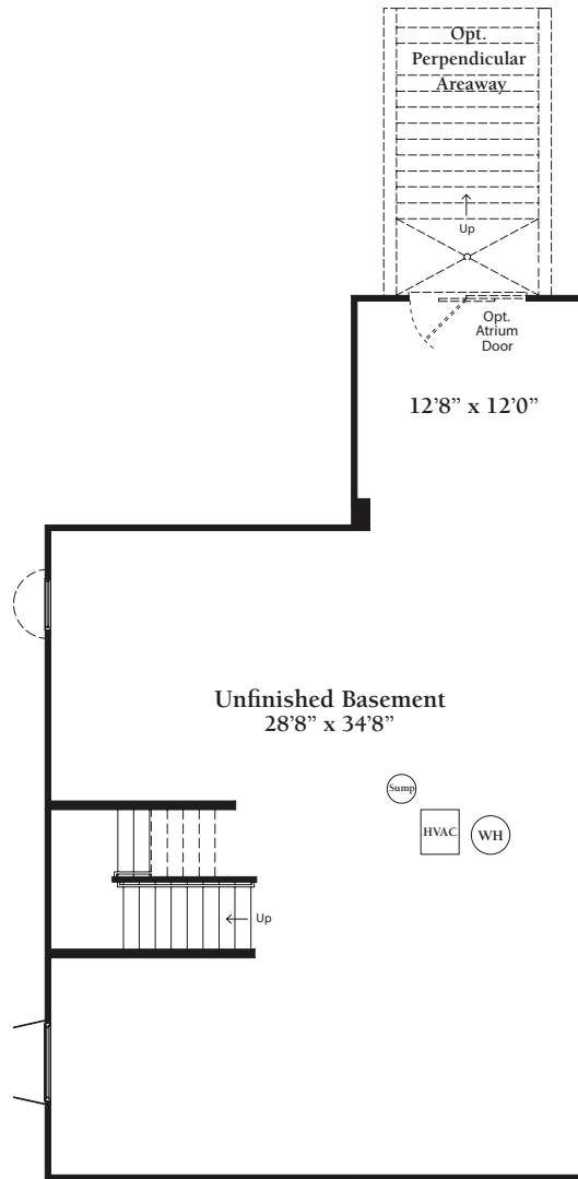
Standard Lower Level Plan Shown w/Opt. Perpendicular Areaway
