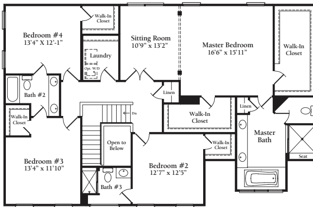
Standard Upper Level Floor Plan
