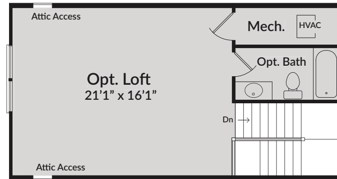
Optional Finished Loft Plan
