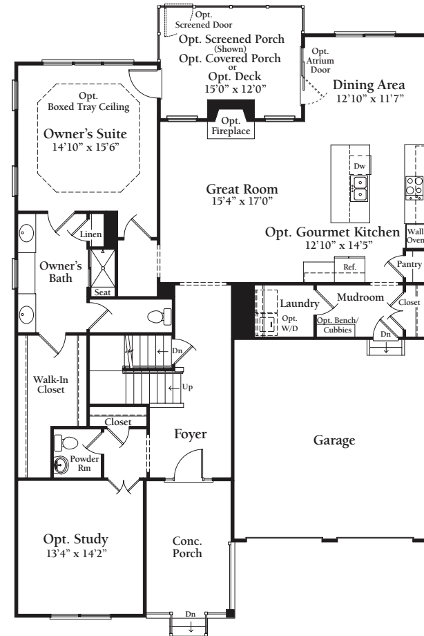
Optional Main Level Floor Plan w/Opt. Gourmet Kitchen, Opt. Fireplace, Opt. Deck or Opt. Screened Porch or Opt. Covered Porch, Opt. Atrium Door, Opt. Boxed Tray Ceiling, Opt. Study, Opt. Cubbies in Mudroom
