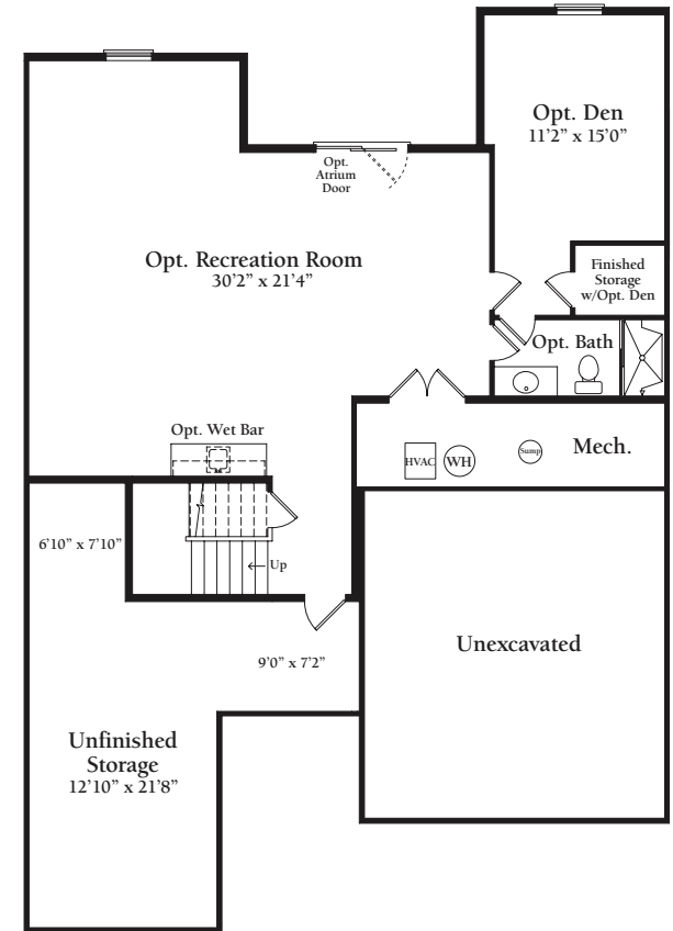
Optional Lower Level Floor Plan w/Opt. Recreation Room, Opt. Den, Opt. Bath, Opt. Wet Bar, Walkout Condition, Opt. Atrium Door
