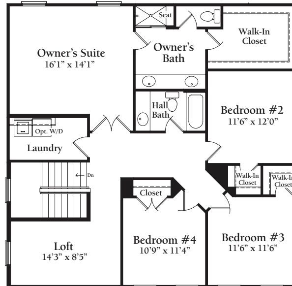
Standard Upper Level Floor Plan
