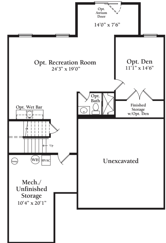
Optional Lower Level Floor Plan w/Opt. Recreation Room, Opt. Den, Opt. Bath, Opt. Wet Bar, Opt. Walkout, Opt. Atrium Door
