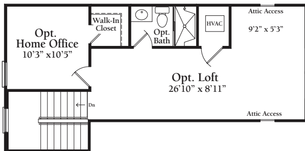
Optional Loft Floor Plan w/Opt. Loft, Opt. Bath, Opt. Home Office
