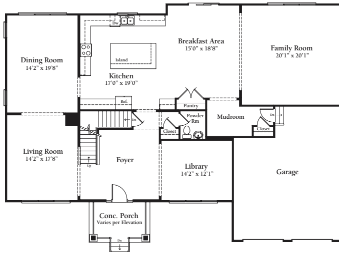
Standard Main Level Floor Plan
