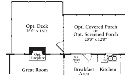
Partial Main Level Plan w/Opt. Fireplace, Opt. Covered Porch or Opt. Screened Porch, Opt. Atrium Door, Opt. Deck
