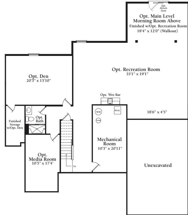
Optional Lower Level Floor Plan w/Opt. 6 Ft. Side Extension, Opt. 4' Rear Extension, Opt. Main Level Morning Room Above, Opt. Recreation Room, Opt. Den, Opt. Bath, Opt. Media Room, Opt. Wet Bar, Opt. Walkout
