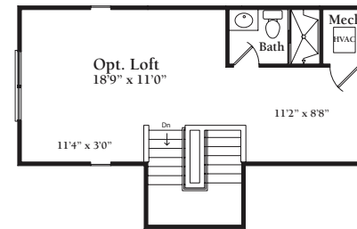
Optional Loft Level Plan w/Opt. Loft with Bath
