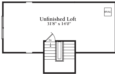
Unfinished Loft Level Plan
