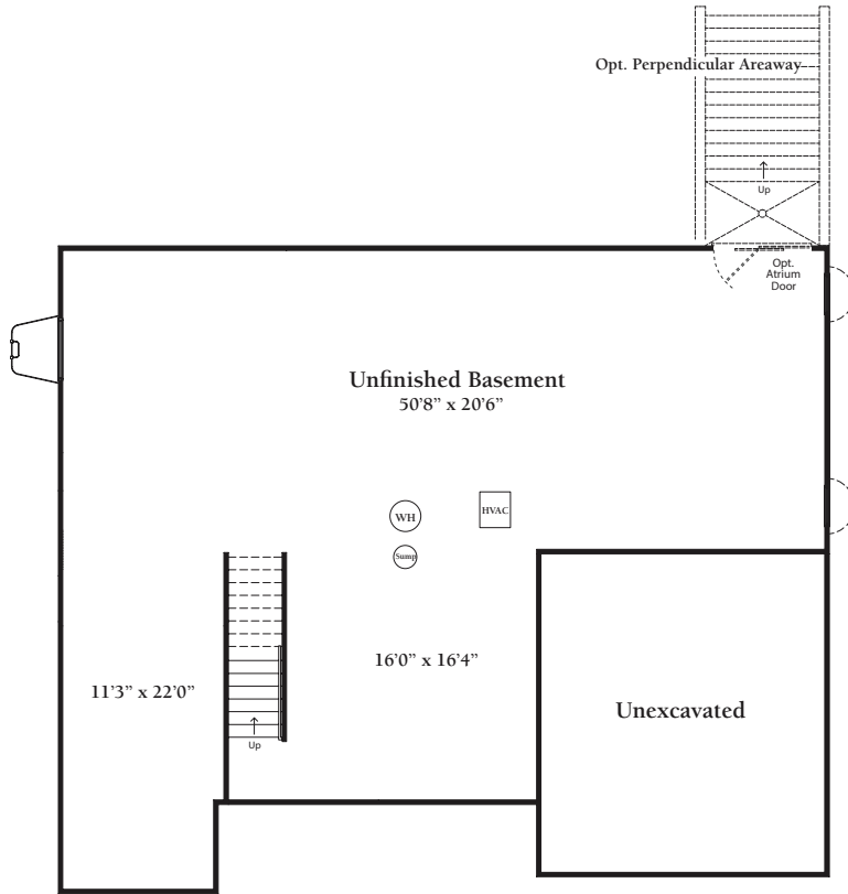
Standard Lower Level Floor Plan Shown w/Opt. Perpendicular Areaway
