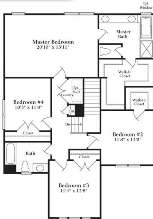
Standard Upper Level Floor Plan
