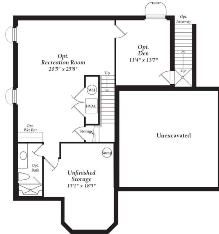
Optional Lower Level Floor Plan w/ Finished Spaces, Opt. Areaway and Opt. Bath
