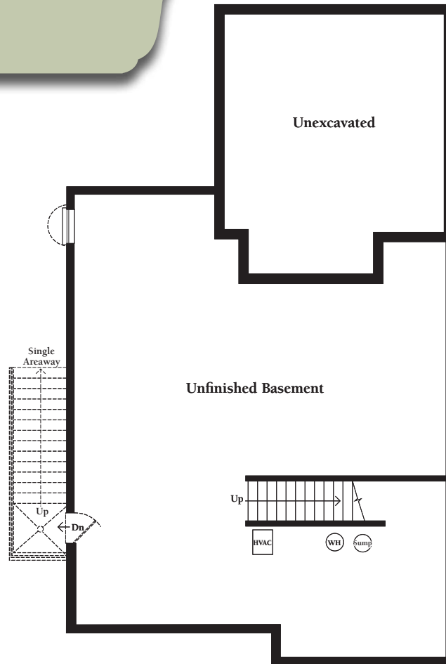
Standard Lower Level Floor Plan w/ Opt. Acreway Elevation C
