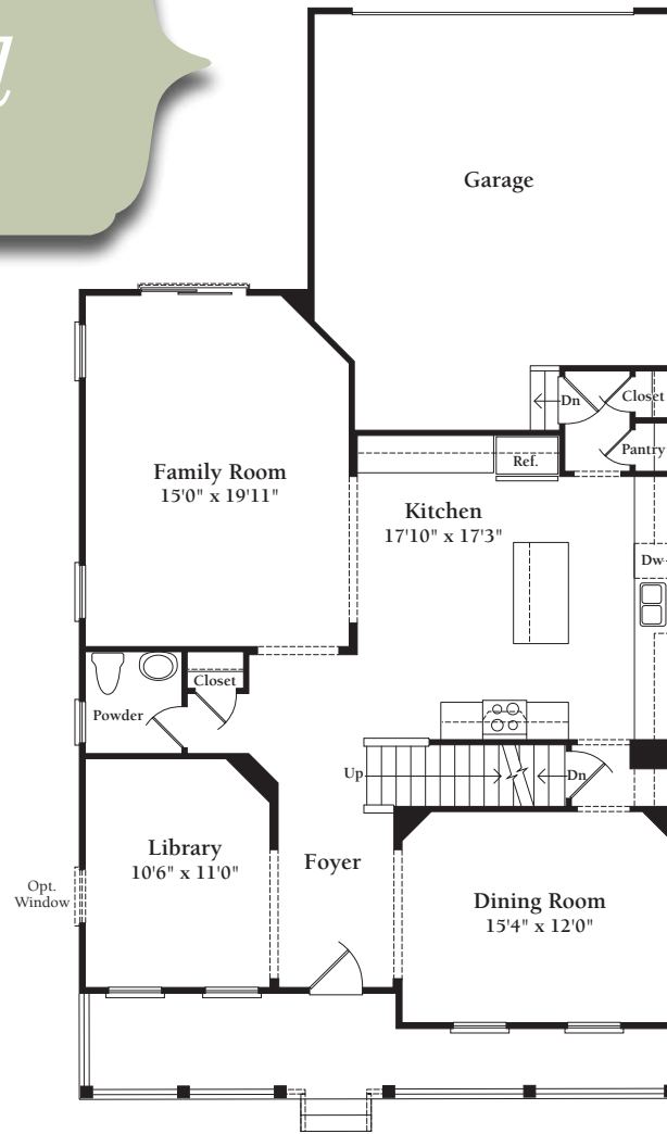
Standard Main Level Floor Plan Elevation C
