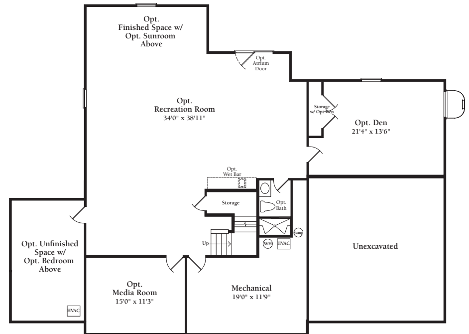
Optional Lower Level Floor Plan w/ Opt. Finished Spaces, Opt. Main Level Sunroom Above, Opt. Guest Suite Above and Breakfast Extension Above, Opt. Walkout Condition and Opt. Wet Bar
