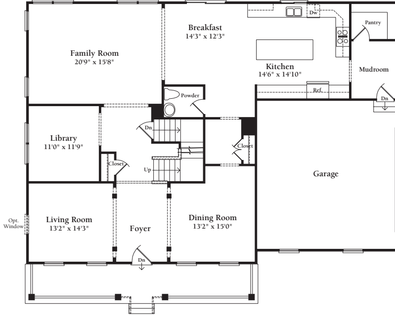
Standard Main Level Floor Plan w/ Side Load Garage Elevation C
