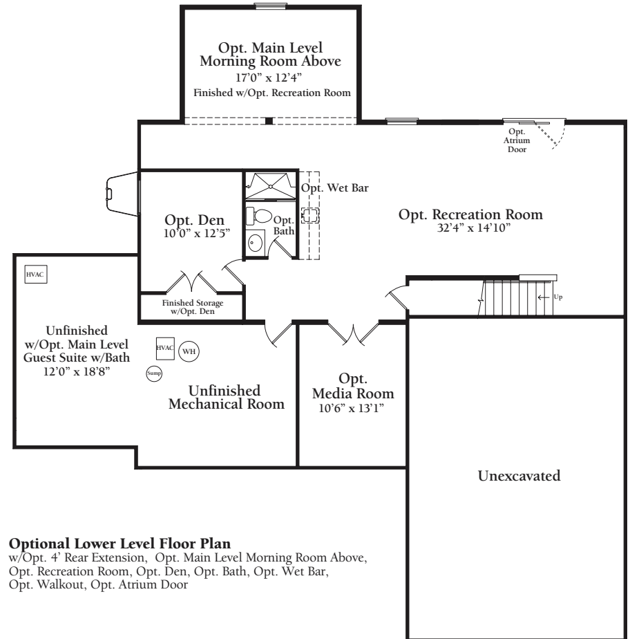
Optional Partial Lower Level Plan
