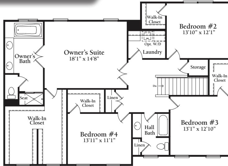
Standard Upper Level Floor Plan
